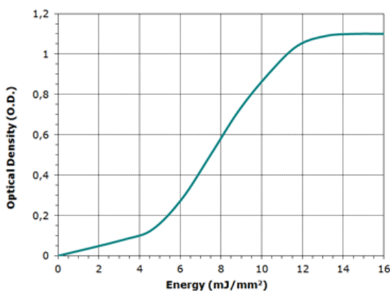
Dynamic Sensitivity
